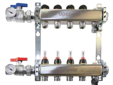
STAINLESS-STEEL MANIFOLD ASSEMBLY
