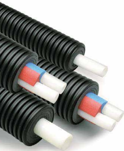
Uponor PRE-INSULATED PIPE
