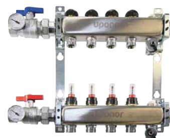
STAINLESS-STEEL MANIFOLD ASSEMBLY
